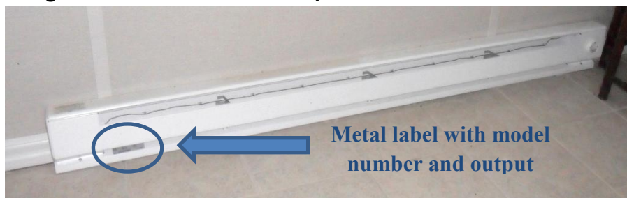
Figure 3-3: Where to Find Output Info for Electric Baseboard
